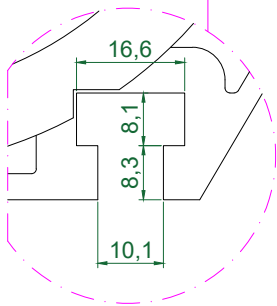
T-Slot Dimensions
